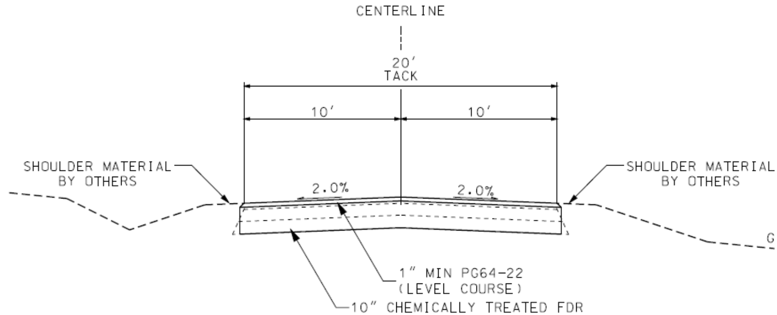
SECTION ON TANGENT TYPICAL SECTION RTE WW LOG MILE 4.414 TO 7.897
